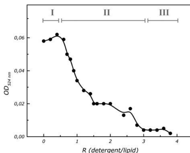
FIGURE 2 Turbidity (optical absorbance at 524 nm) of egg PC liposomes at various LDAO to egg PC ratios. The effect of the detergent on the physical state of the liposomes can be followed. The three indicated stages are discussed in the text.
