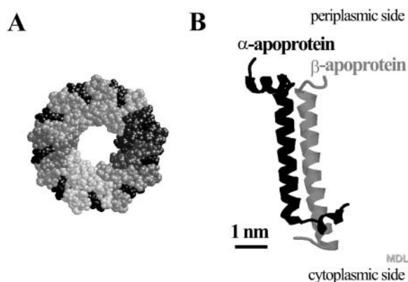
FIGURE 1 (A) Topology model (top view, periplasmic side) of the LH2 of Rps. acidophila strain 10050. It consists of a concentric arrangement of two hollow cylinders built from nine \alpha - and nine \beta -apoproteins. The outer surface of the cylinder is formed by the \beta -subunits, and its inner surface by the \alpha -subunits. Each \alpha\beta -apoprotein pair binds four pigment molecules, three bacteriochlorophylls, and two carotenoid molecules. The spheres in various shades of gray represent the 18 apoproteins and the black spheres represent the pigment molecules. (B) Topology model of an \alpha\beta -apoprotein pair without the associated pigment molecules. Model A has been scaled down five times with respect to Model B.
